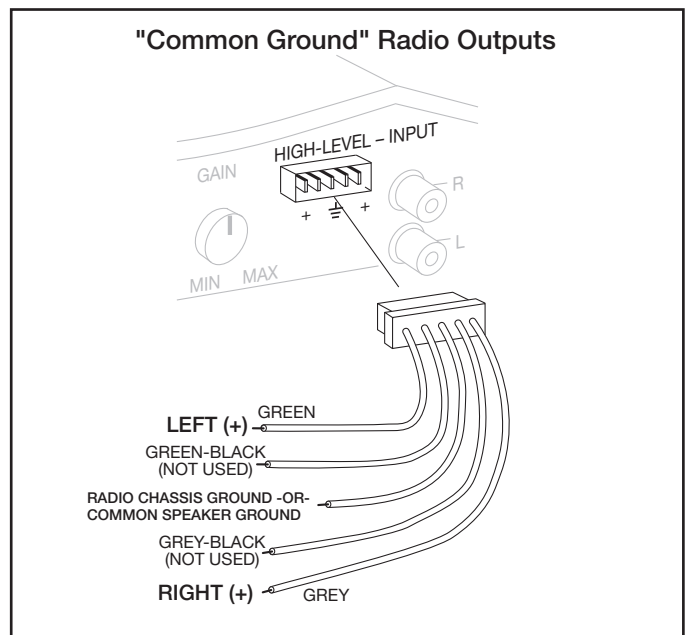
High Level (Speaker Input) Wiring
